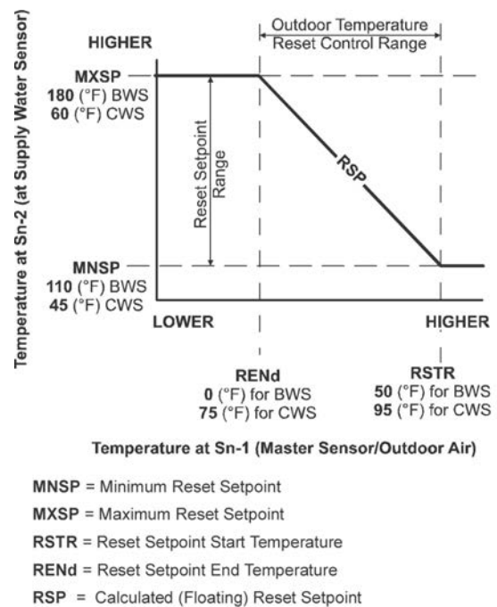
Figure 3: Reset setpoint application for boiler water supply (BWS) and chiller water supply (CWS) showing relationships between the reset
