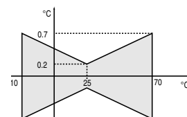
Misura di temper. (Pt1000), range -10...70°C
