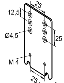
Extension bracket Part No.: 803 800
