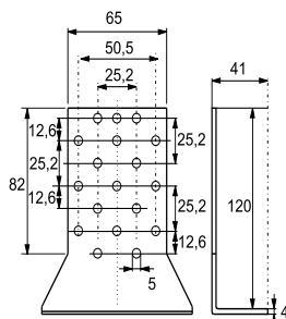
Universal mounting bracket Part No.: 803 798
