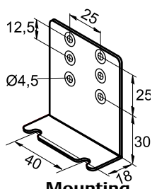
Mounting bracket angle Part No.: 803 799
