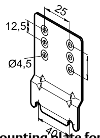
Mounting plate for units with hood Part No.: 803 801
