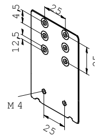
Extension bracket Part No.: 803 800
