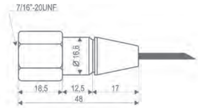
FEMALE FITTING
