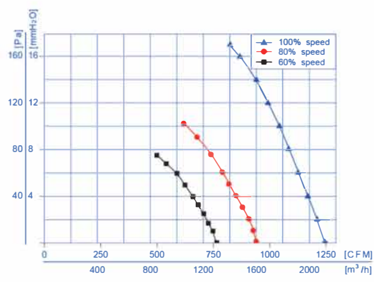
FLOW RATE CURVE :
